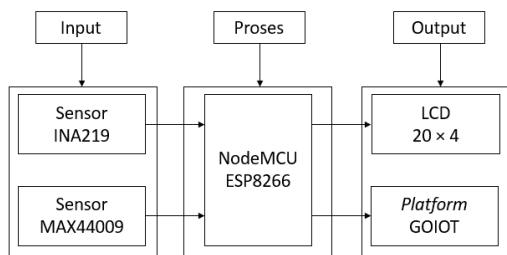
Gambar 1. Diagram Blok Sistem Monitoring Solar Tracker
