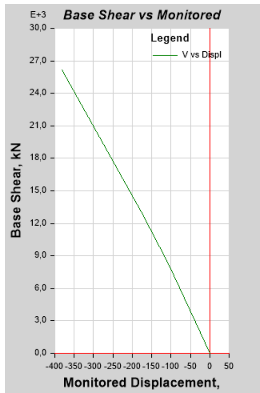
Figure 3. Capacity curve in x and y directions
