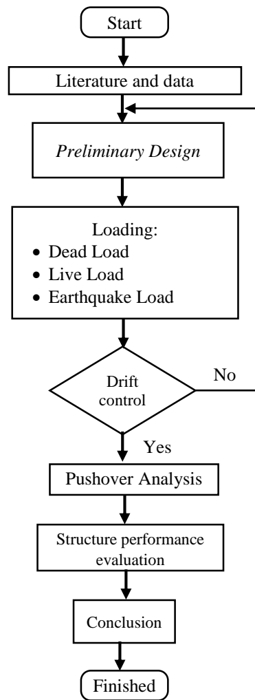
Figure1. Flow Chart
