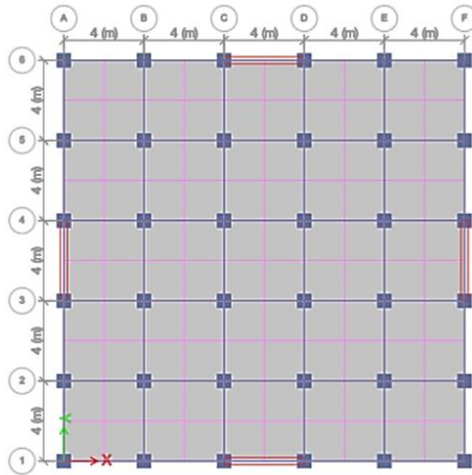
Figure 2. Top View of the Building
